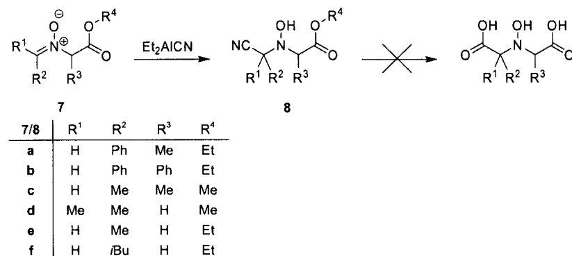
Scheme 1. Attempts to obtain amavadin ligand analogues by the addition of cyanide to nitrones.
