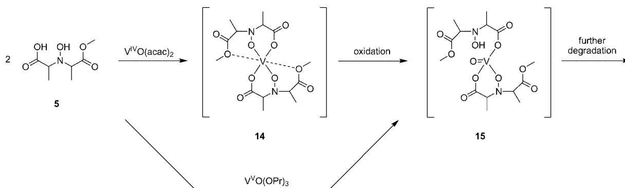
Scheme 6. Schematic representation of the tentative V IV and V V complexes formed from ligand 5 .
