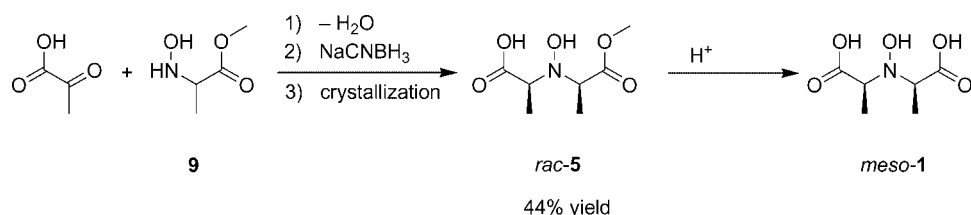
Scheme 3. Synthesis of bidentate ligand 5 and meso - 1 .
