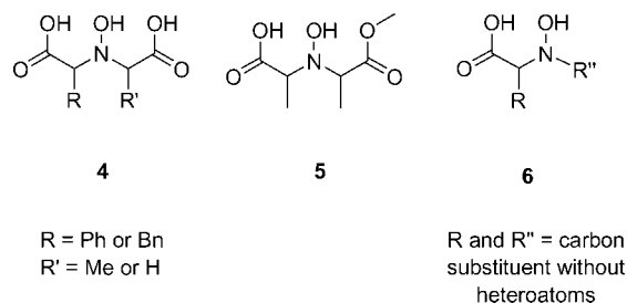
Figure 2. Amavadin-based ligands 4–6 .
