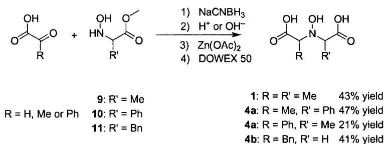
Scheme 2. Synthesis of tridentate ligands 4 .
