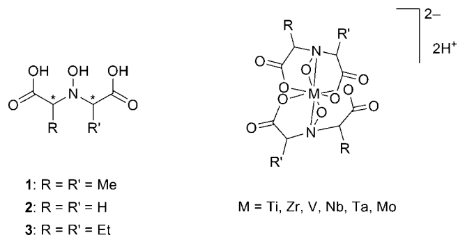
Figure 1. Amavadin analogues 1–3 reported in the literature.
