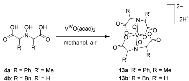
Scheme 5. Formation of the amavadin analogues 13a and 13b from ligands 4a and 4b .
