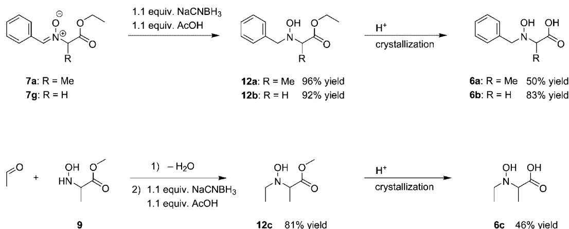
Scheme 4. Synthesis of bidentate ligands 6 .
